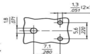
Mounting layout
