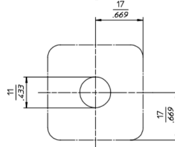
Mounting layout
