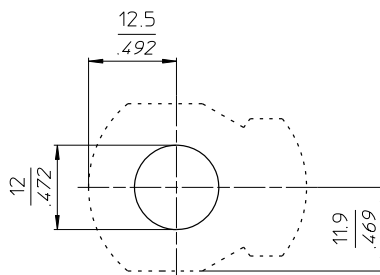
Mounting layout
