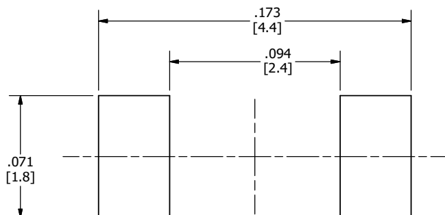
SUGGESTED FOOTPRINT SOLDER PASTE THICKNESS OF 0.15 [mm] RECOMMENDED
