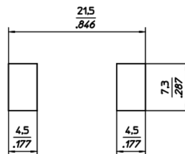
Mounting layout
