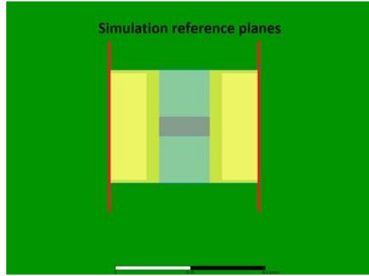
Reference planes for the simulation are at the edge of the component pad stack. Reference plane separation 12mils.
