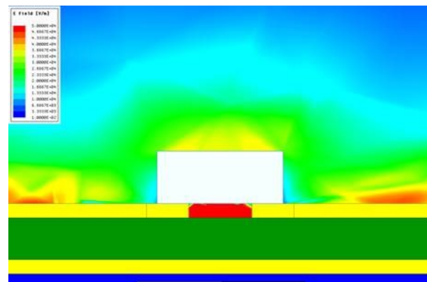
E-Field Visualization
