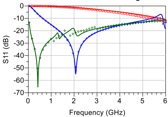
60 mil Rogers 4003C (H/Er = 16.7 mil):
